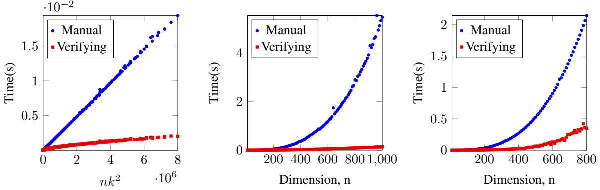
(a) Matrix Multiplication of A \in \mathbb{F}_q^{k \times n} and B \in \mathbb{F}_q^{n \times k} and 500 runs per test, for n and k from 10 to 200. (b) Eigen-decomposition of symmetric A \in \mathbb{F}_q^{n \times n} with \epsilon = 0.01 and 150 runs per test. (c) Matrix Inversion of A \in \mathbb{F}_q^{n \times n} where \epsilon = \frac{1}{2} and 100 runs per test.
