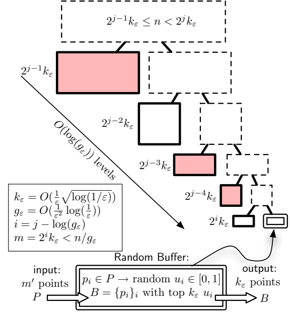
Figure 1: Illustration of the hybrid summary. The labels at each level of the hierarchy shows the number of points represented at that layer. Each filled box contains only k_\varepsilon summary points.
