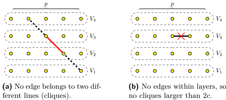
Figure 4 Clique gadget proof sketch for Theorem 7.
