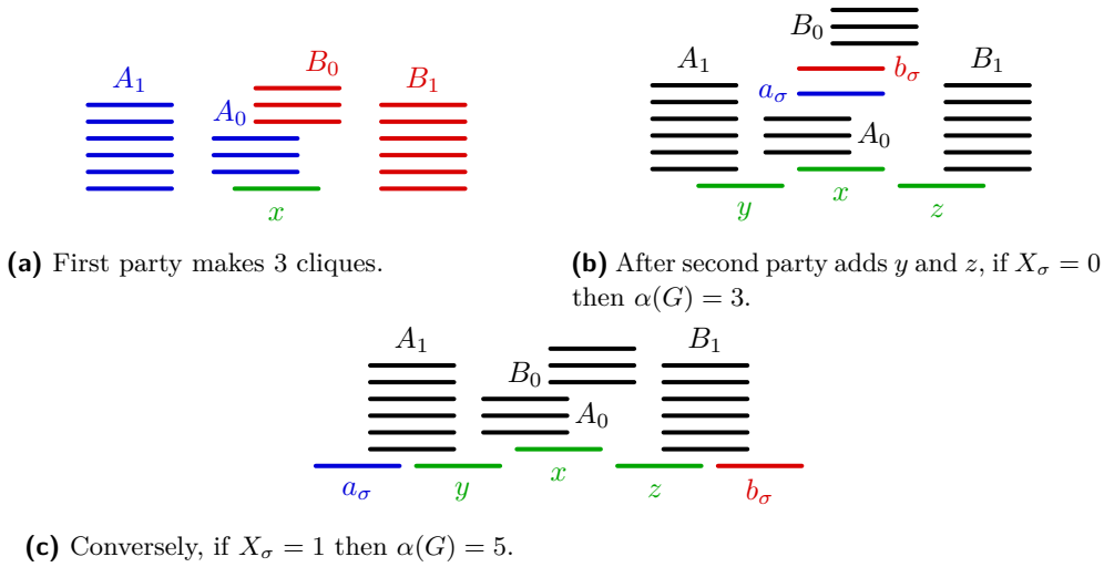
■ Figure 6 Interval representations for the construction in theorem 18. Horizontal positioning represents the location of the intervals in \mathbb{R} , vertical positioning is for clarity only.
