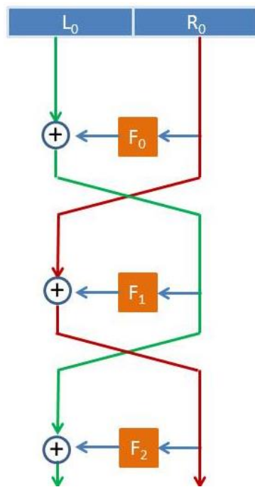
Three-round Feistel Network with group operation +
