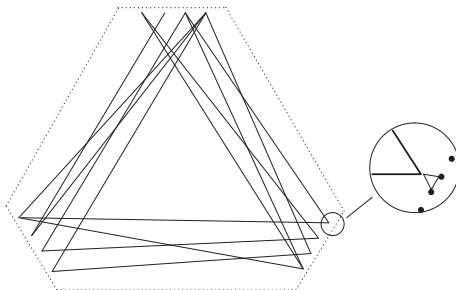
Figure B.1: The reduction for a 3-partite graph on 12 vertices.
