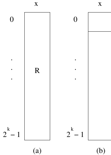
Figure 6: Example showing the deficiencies of PAR definitions based on probability mass.
