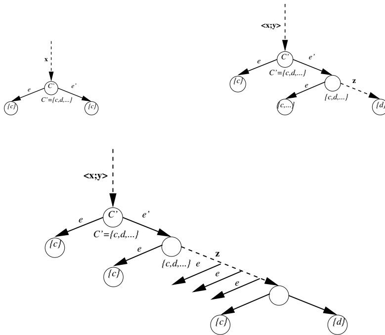
Figure 2: Illustration of proof of Lem. F.8.
