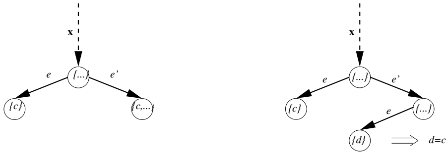
Figure 1: Illustration of the two conditions of loD.
